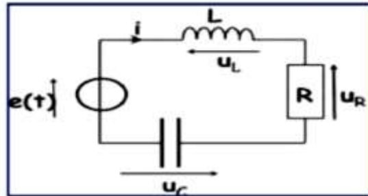
Figure 2: Circuit RLC
