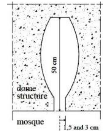
Fig 21: Cross section of the resonators found in the dome of the Sultan Ahmet Mosque dôme (Source: Kayili, M. (2005))
