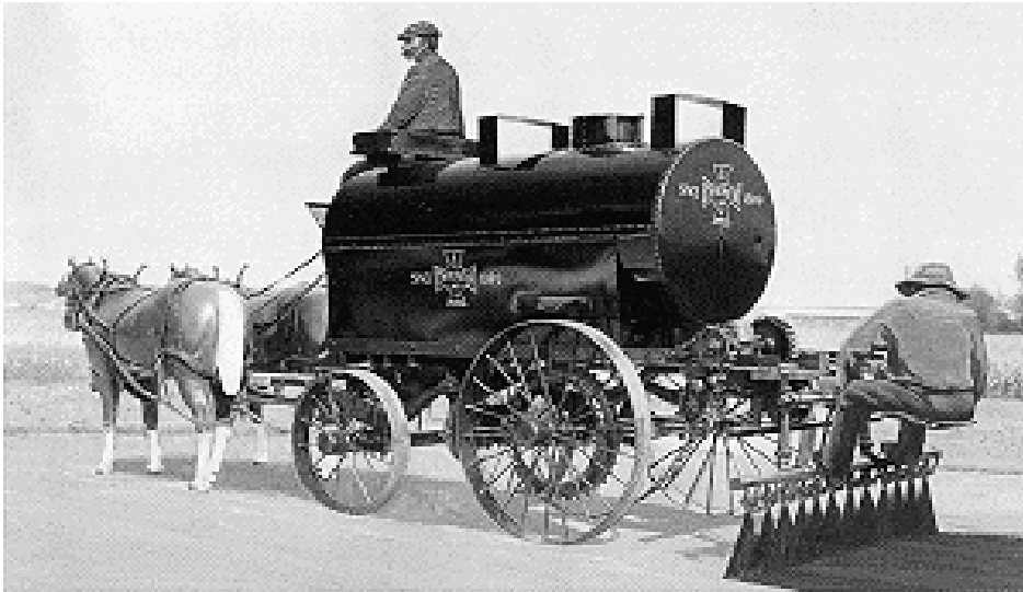
Macadamization of roads
